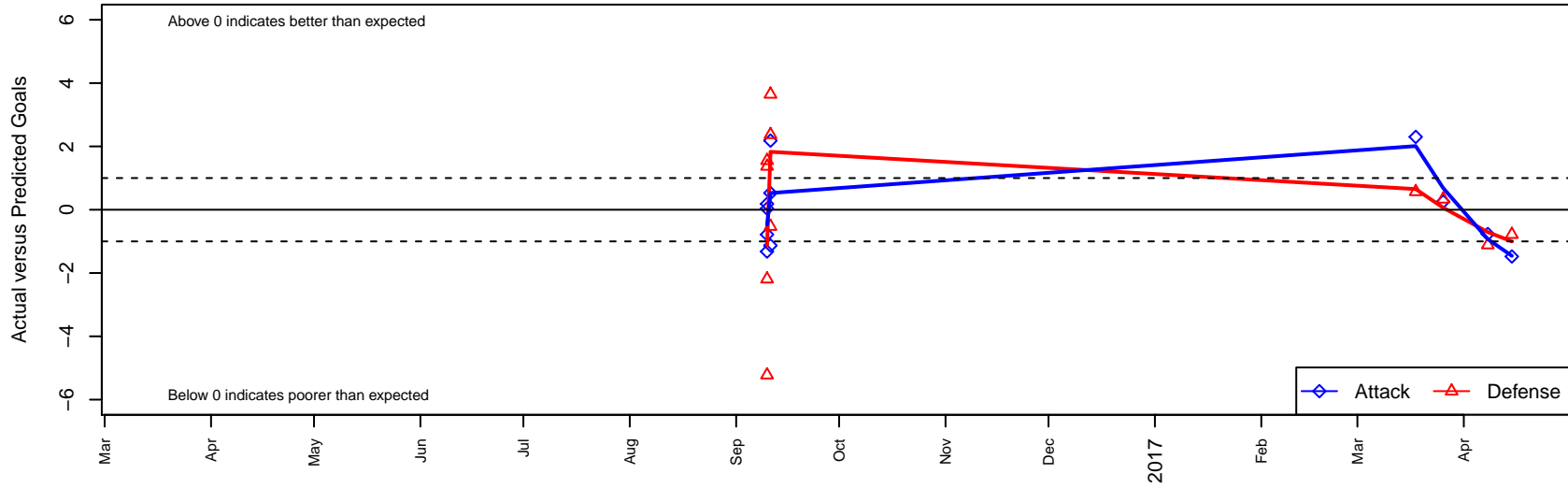
Valley Thunder SC G05 Dots are actual minus expected GF (blue circles) and GA (red triangles). Blue line is smoothed change in attack strength. Red is smoothed change in defense strength.
